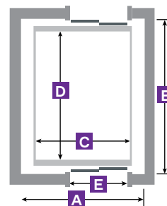
Top view: Front and rear opening
