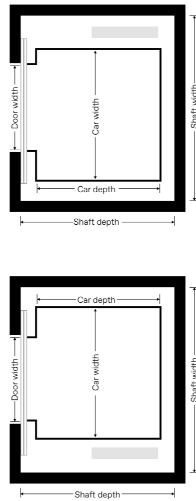
Lift plan
